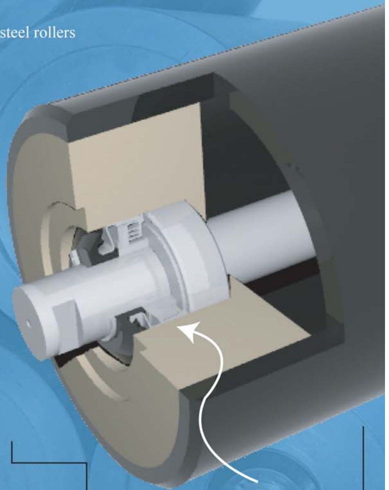
Multi-Labyrinth seal, see below for detail
